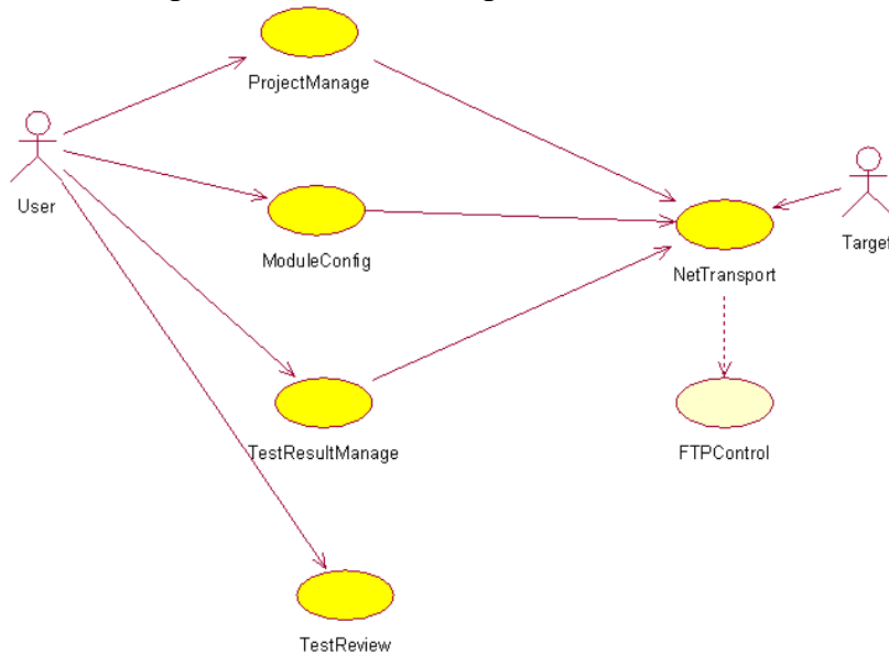
Figure 4. system use case diagram
