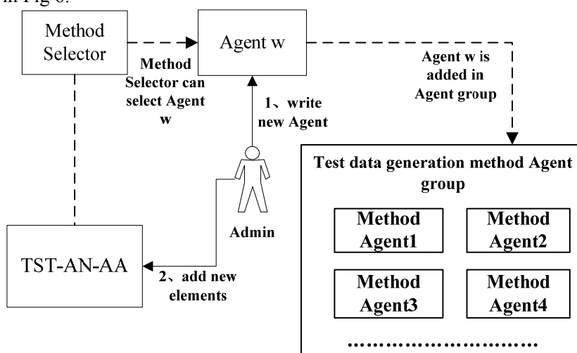
Figure 6. principle of software test data generation method extension
