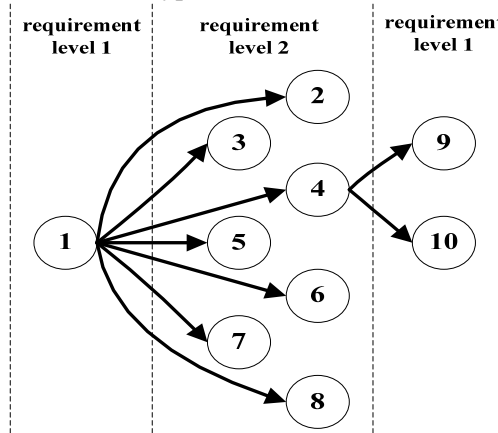
Fig 5 Test requirement tree
