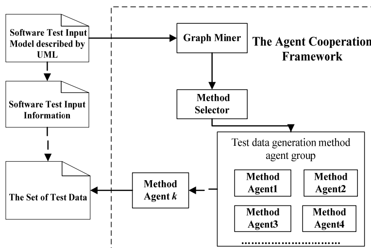
Figure 2. Agent cooperation framework
