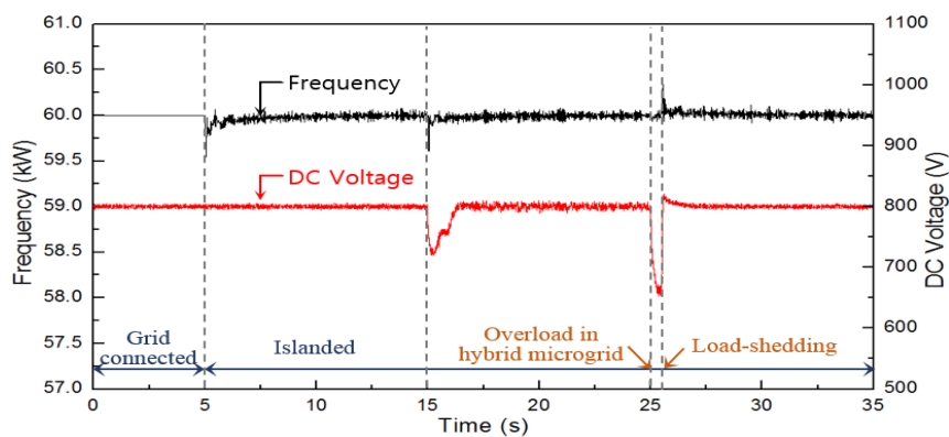
Figure 14. Frequency and DC Voltage in the Hybrid Microgrid
