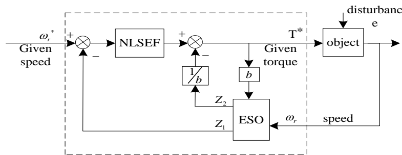
Figure 5. The Structure of Speed Controller based on ADR
